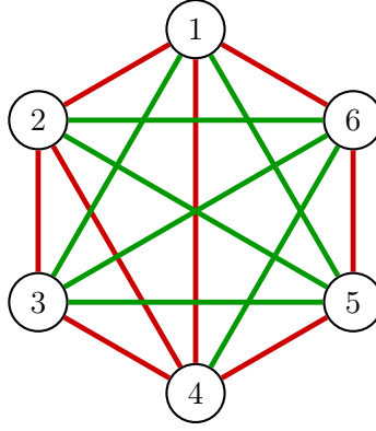
Figure 1: An example 2 colour colouring fulfilling Ramsey number R(3, 3) = 6 . Nodes 1, 3, 5
